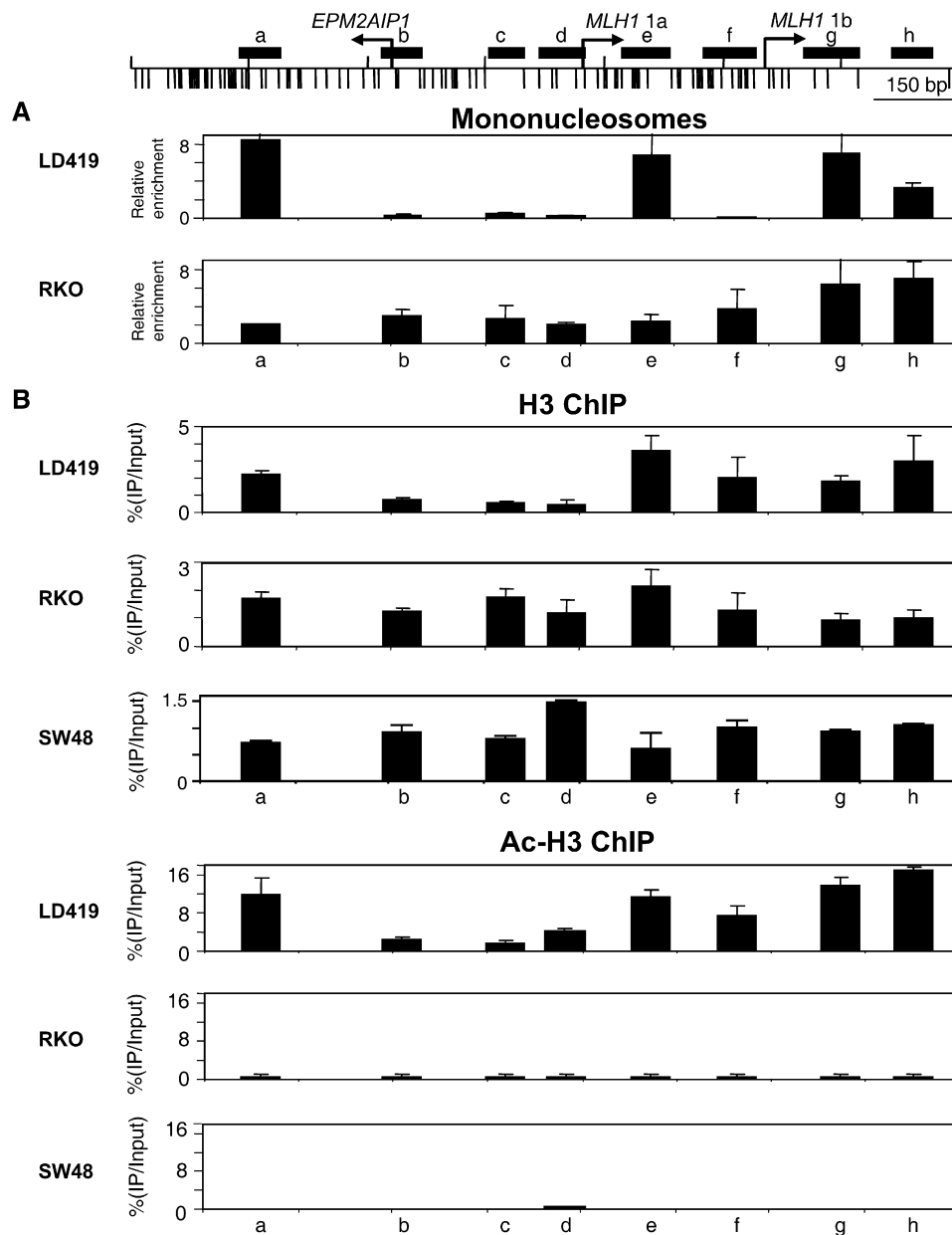
Figure 3. Nucleosomal Depletion by Mononucleosomal DNA and ChIP Analyses
