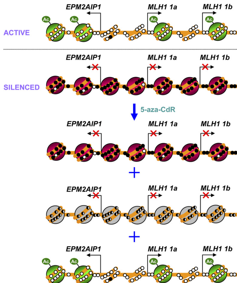
Figure 8. A Simplified Model for the Epigenetic Silencing of the MLH1 Gene
