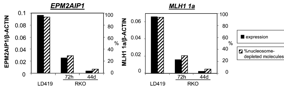
Figure 7. Correlation between the Expression Level and the Percentage of Nucleosome-Depleted Molecules
